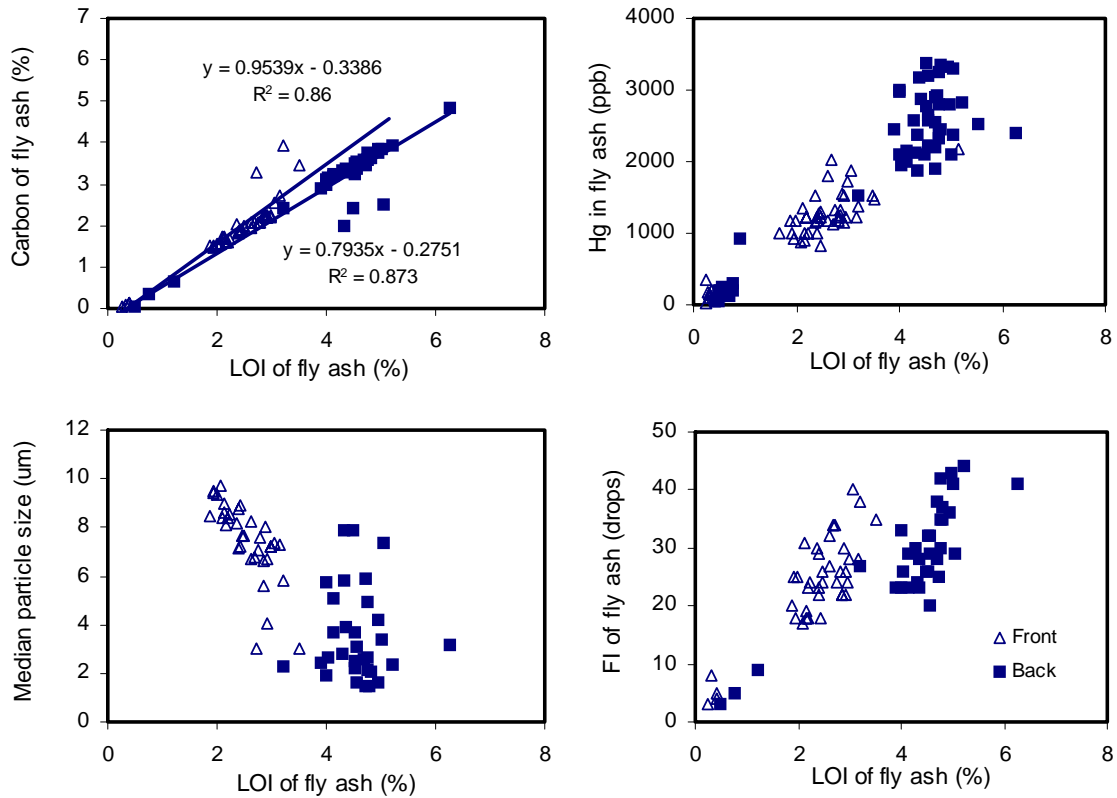
Figure 6. Correlations of mercury, carbon, LOI, particle size, and MB-VR FI of fly ash. All samples are composite.
